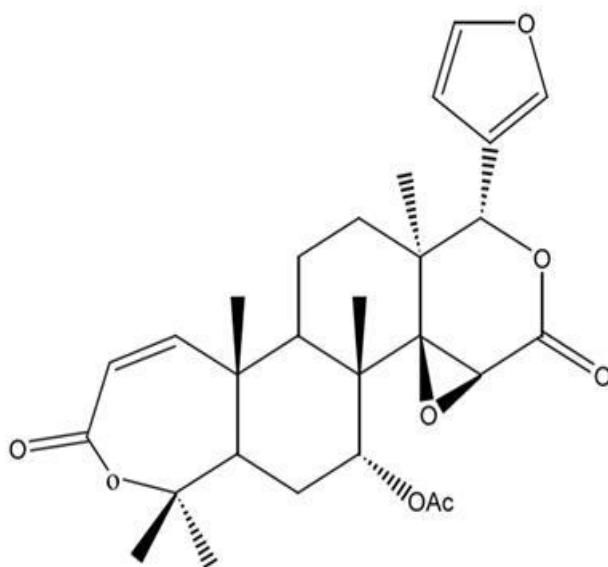
Figure 6: Terpenoid structure
